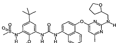
N-{5-tert-Butyl-2-methoxy-3-[3-(4-{6-methyl-2-[(tetrahydrofuran-2-ylmethyl)-amino]-pyrimidin-4-yloxy}-naphthalen-1-yl)-ureido]-phenyl}-methanesulfonamide;
